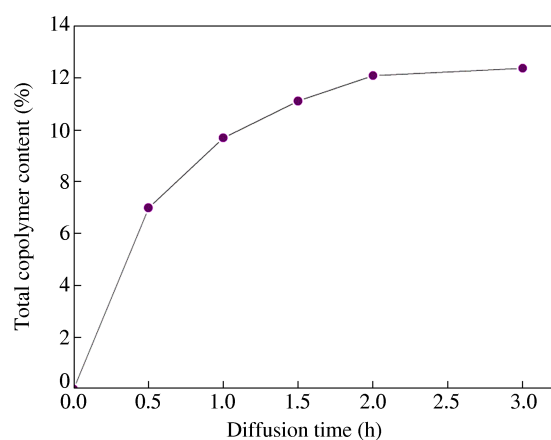
Fig. 2 Total copolymer content as a function of diffusion time with a comonomer feed ratio St:BMA 1:1
